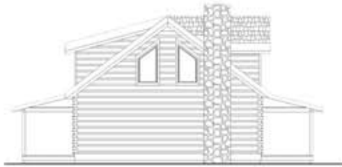
LEFT ELEVATION
